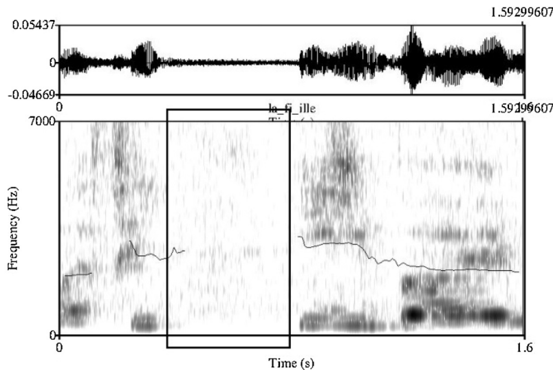
Fig. 9. Waveform and spectrogram for the disfluency ‘la fi-ille’ [la fi#ij].
