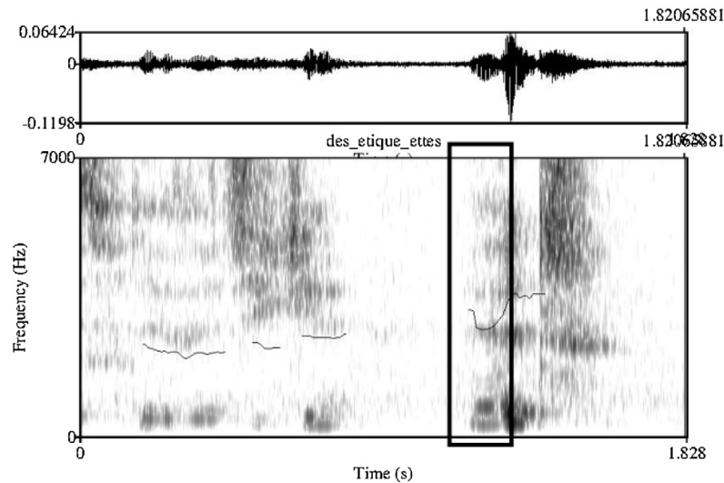
Fig. 8. Waveform and spectrogram for the disfluency “des étiquettes” [dezetikɛ # hɛt].
