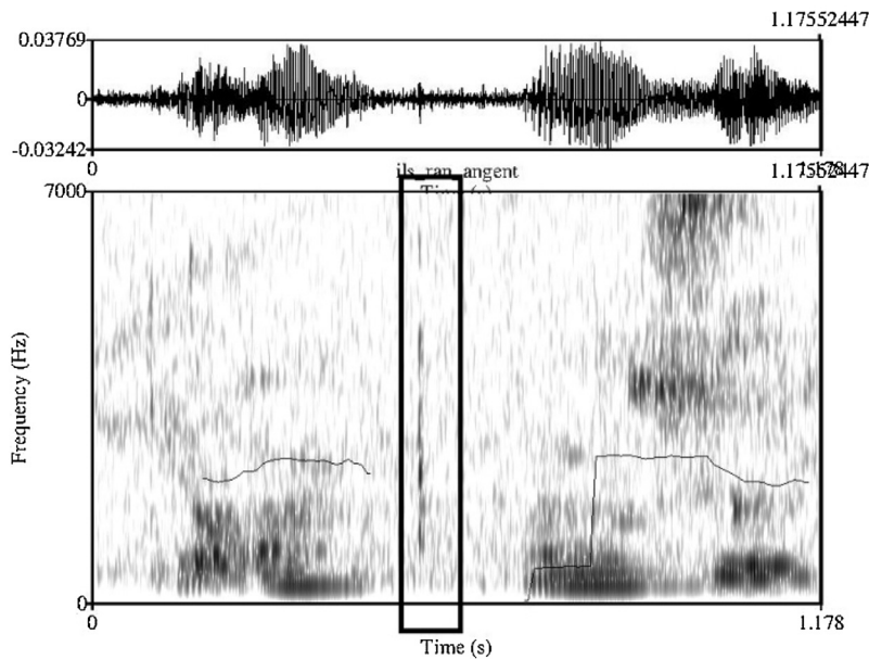
Fig. 7. Waveform and spectrogram for the disfluency “ils ran-angent” [ilʁ ãʔ # ã ʒã].
