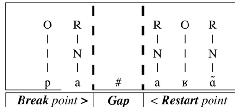
Fig. 1. Formalisation of the disfluencies' classification (O = Onset, R = Rhyme, N = Nucleus), example: 'parents' [pa-aʁɑ̃].
