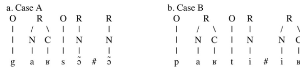
Fig. 2. Syllabification of disfluencies before nuclei in word final position: cases A and B (O = Onset, R = Rhyme, N = Nucleus, C = Coda).
